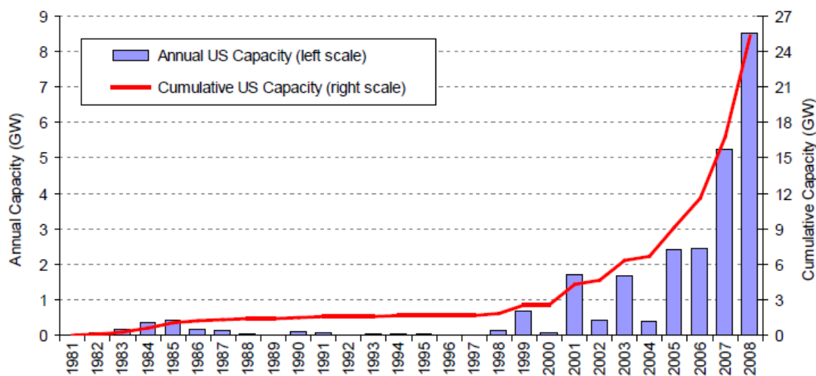
Figure 2-7: Annual and cumulative growth in U.S. wind power capacity (Source: EERE [8])
